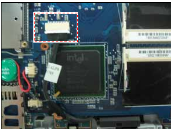
Step 56. Disconnect the IR Board HARNESS.
